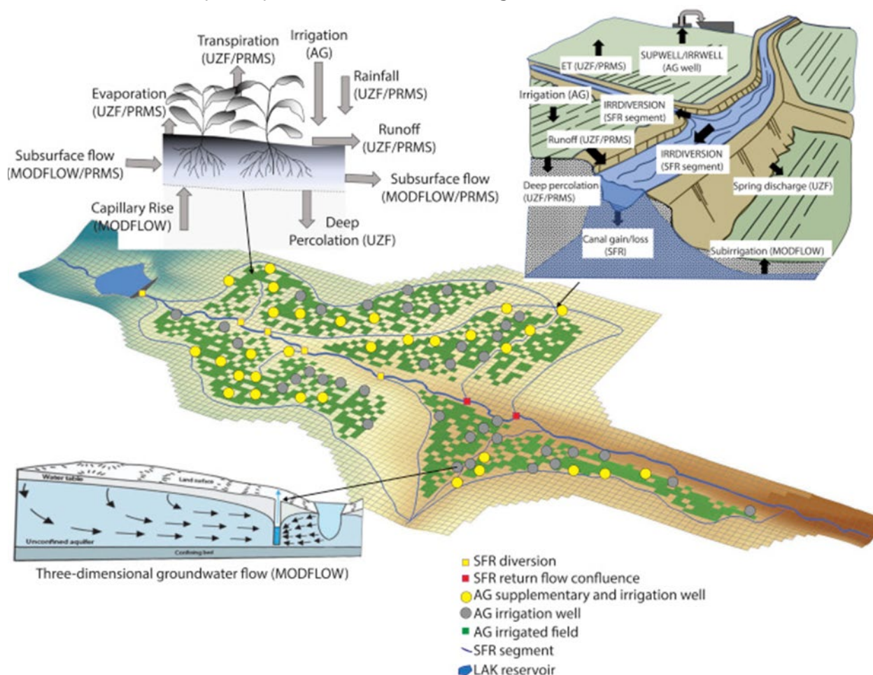
Figure E-2. Illustration Showing How the Agricultural Water Use Package Represents Agricultural Processes in MODFLOW, PRMS, and GSFLOW (from Niswonger 2020)
