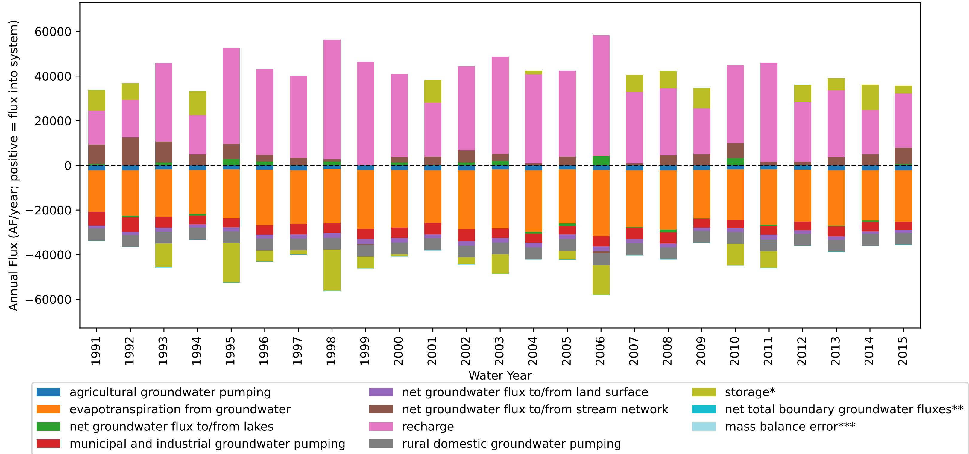
Upper Russian River subbasin Annual Groundwater Water Budget, WY 1991-2015
