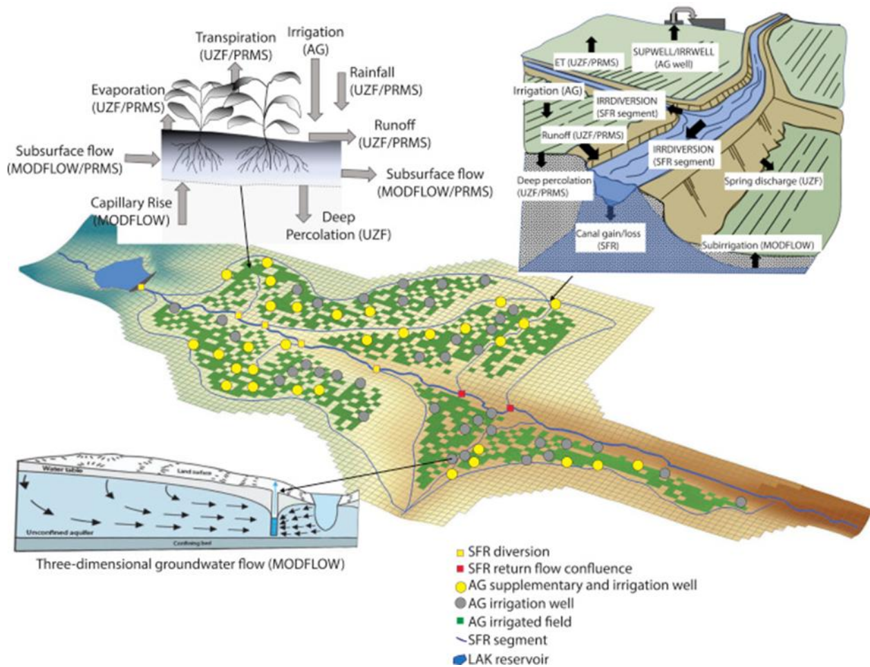
Figure E-2. Illustration Showing How the Agricultural Water Use Package Represents Agricultural Processes in MDOFLW, PRMS, and GSFLOW (from Niswonger, 2020)
