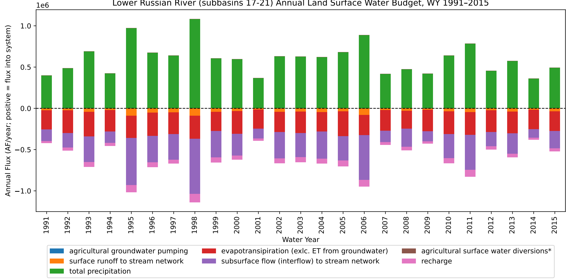
Lower Russian River (subbasins 17-21) Annual Land Surface Water Budget, WY 1991-2015
