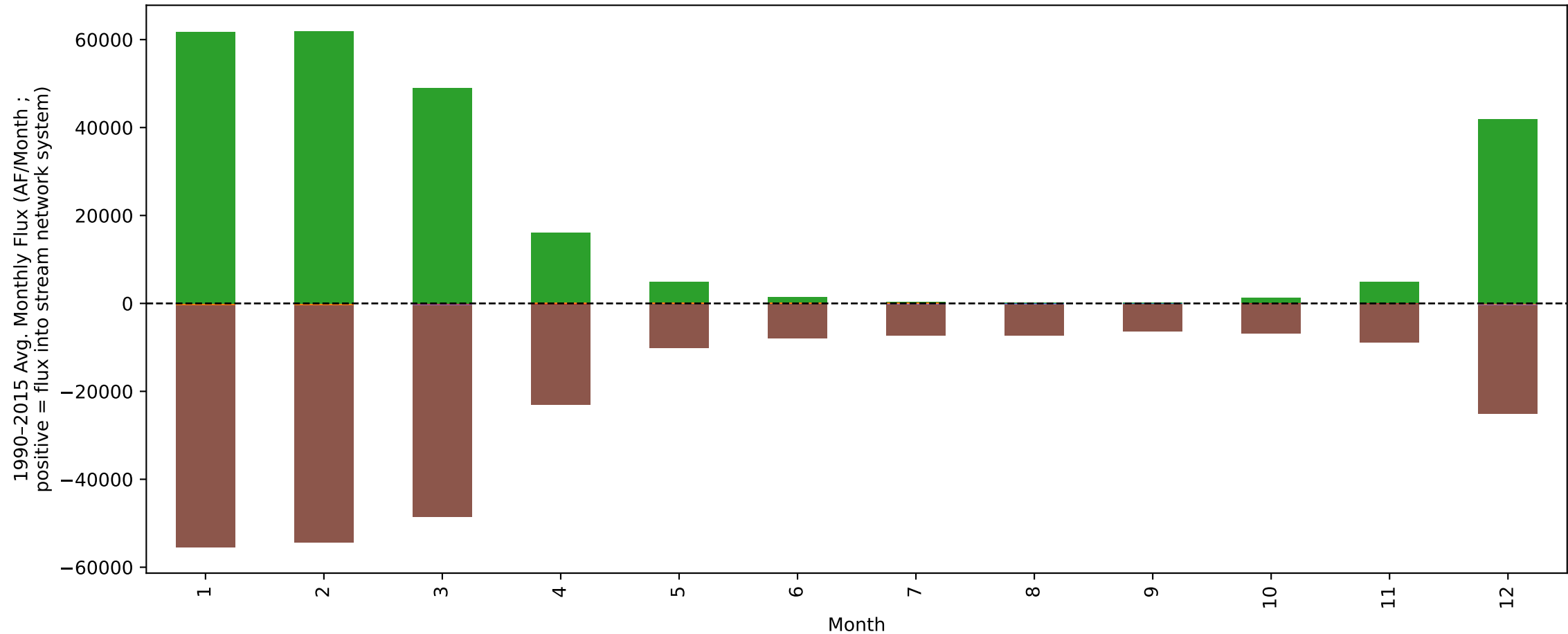
Dry Creek (subbasins 14-16, 22) Monthly Avg. Stream Network Budget
