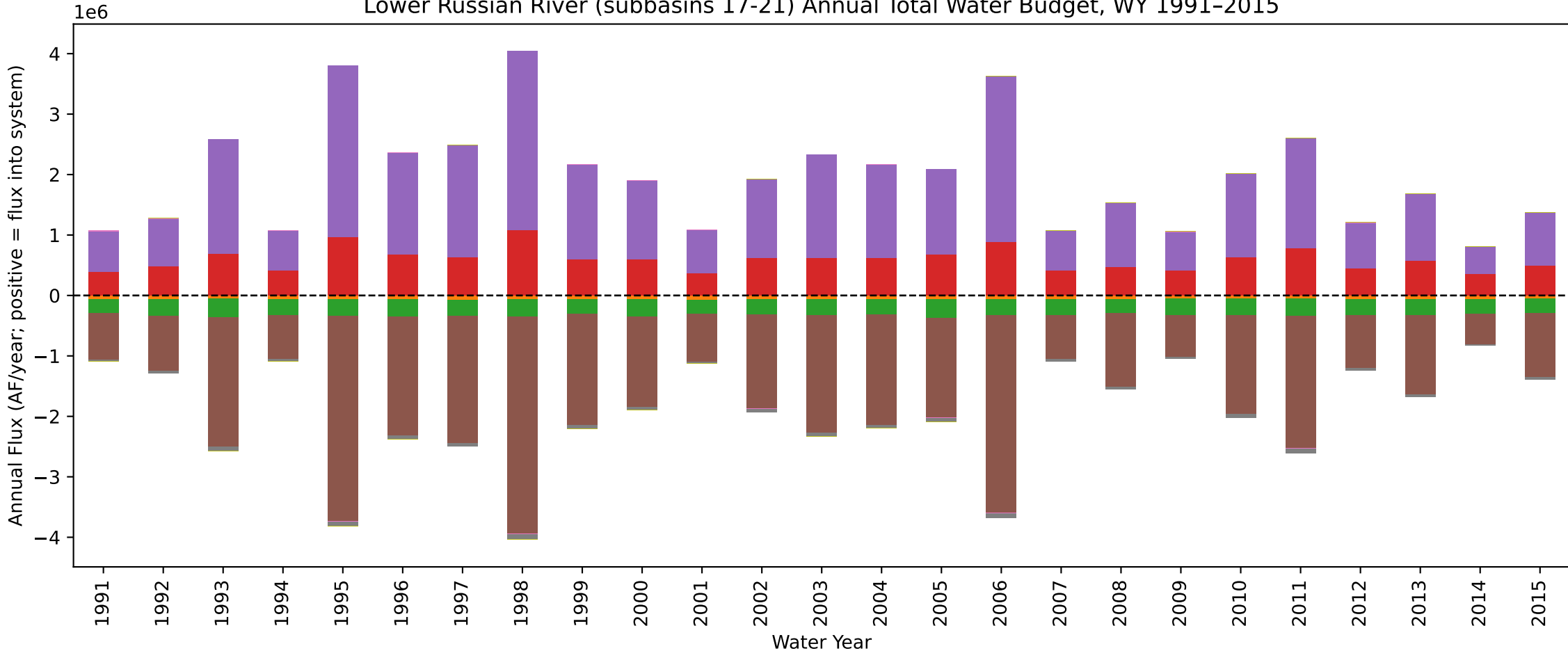
Lower Russian River (subbasins 17-21) Annual Total Water Budget, WY 1991-2015
