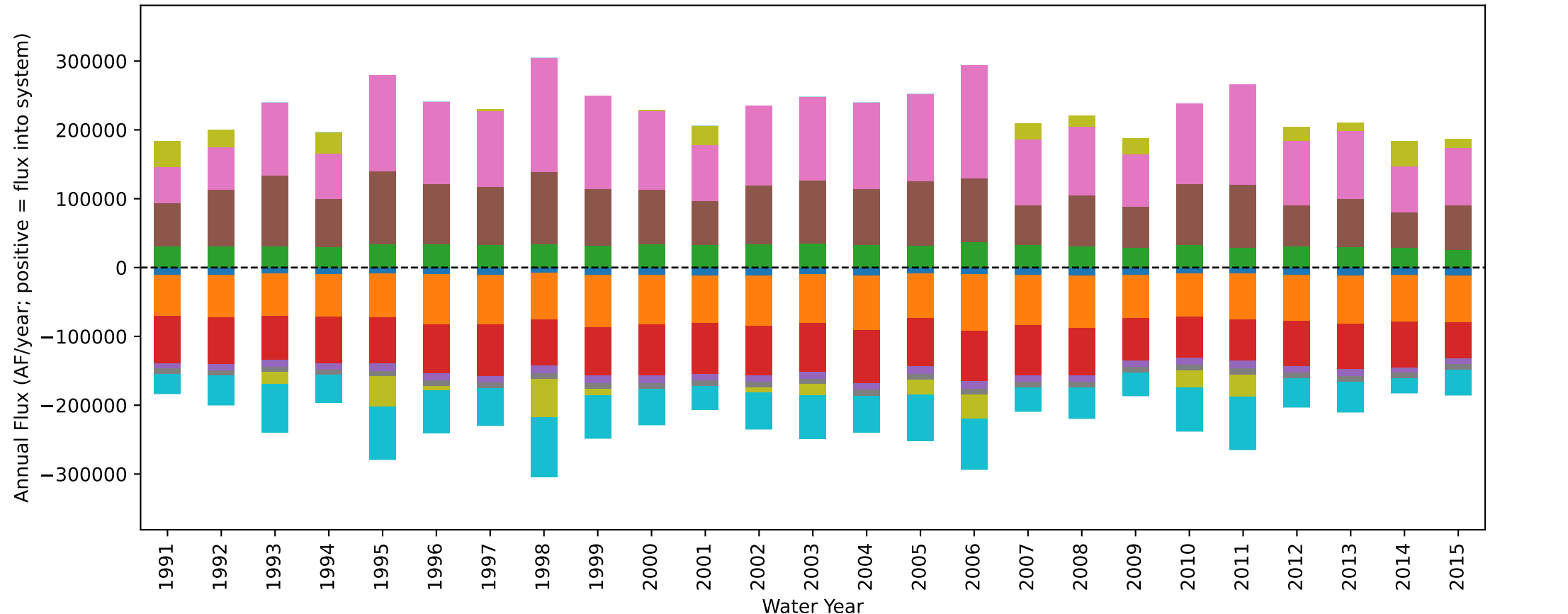
Russian River Watershed Annual Groundwater Water Budget, WY 1991–2015
