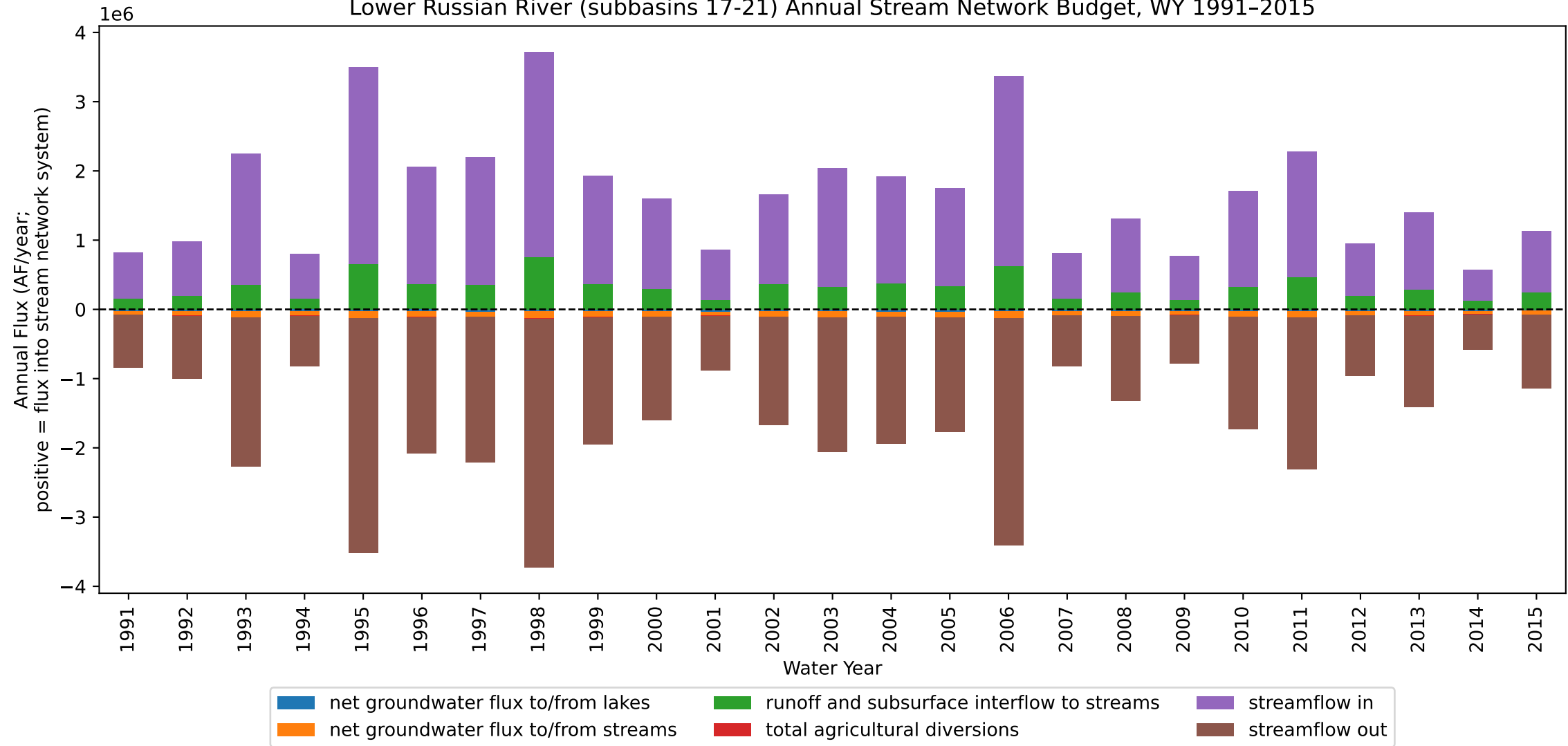
Lower Russian River (subbasins 17-21) Annual Stream Network Budget, WY 1991-2015
