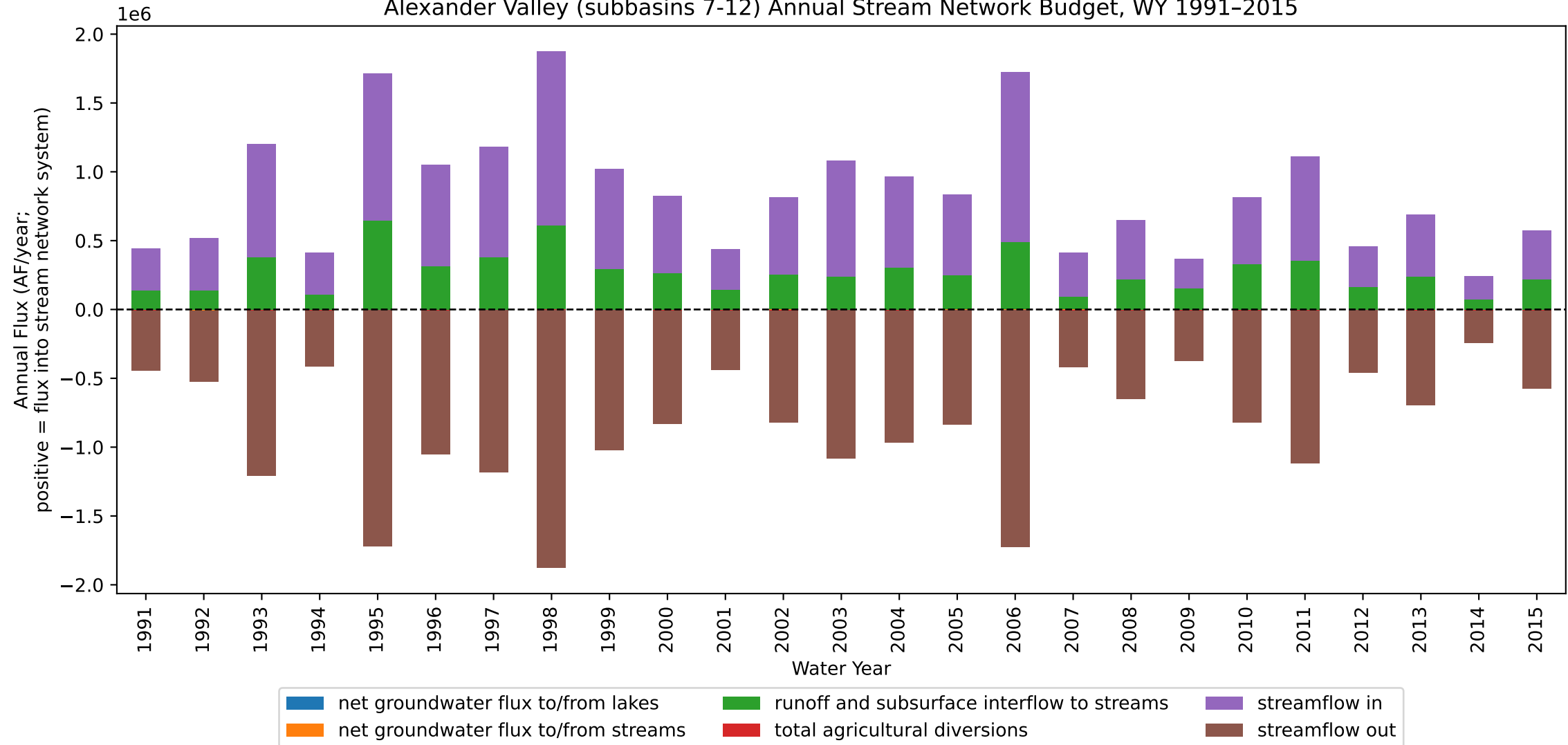
Alexander Valley (subbasins 7-12) Annual Stream Network Budget, WY 1991-2015
