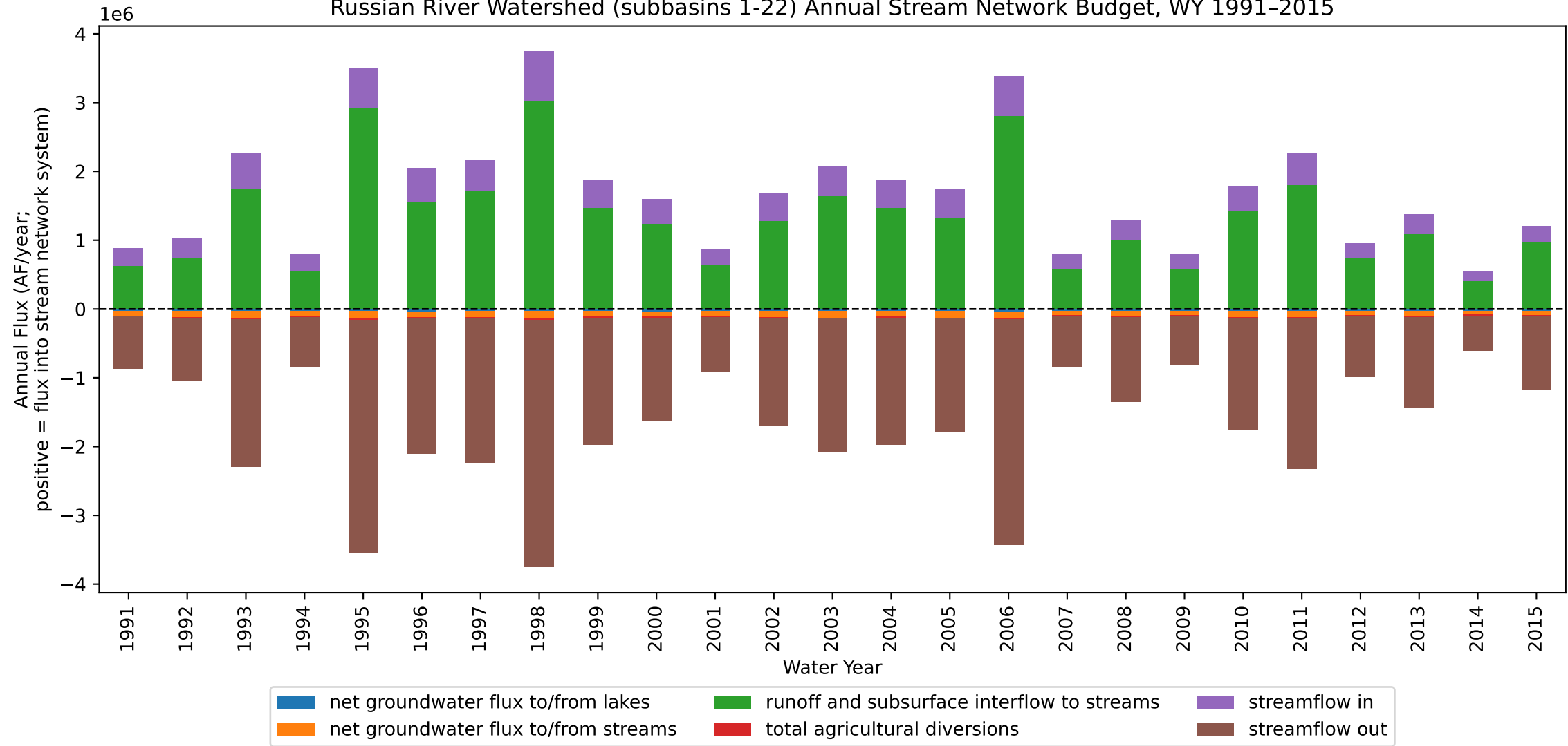
Russian River Watershed (subbasins 1-22) Annual Stream Network Budget, WY 1991-2015
