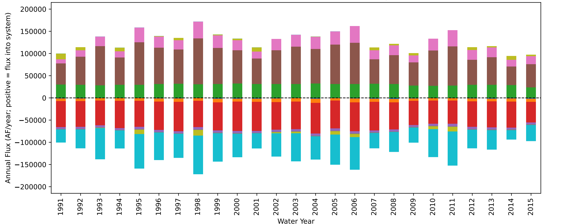
Lower Russian River subbasin Annual Groundwater Water Budget, WY 1991-2015
