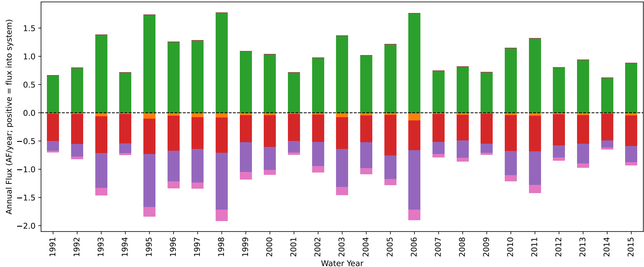
Upper Russian River (subbasins 1-6) Annual Land Surface Water Budget, WY 1991-2015
