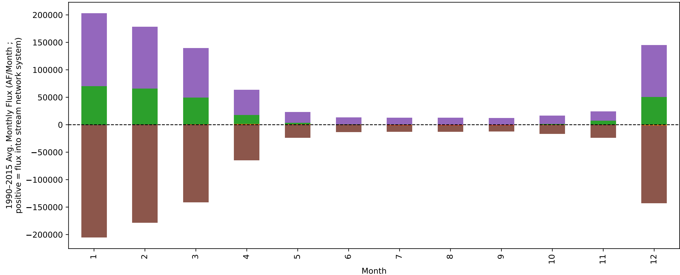
Alexander Valley (subbasins 7-12) Monthly Avg. Stream Network Budget
