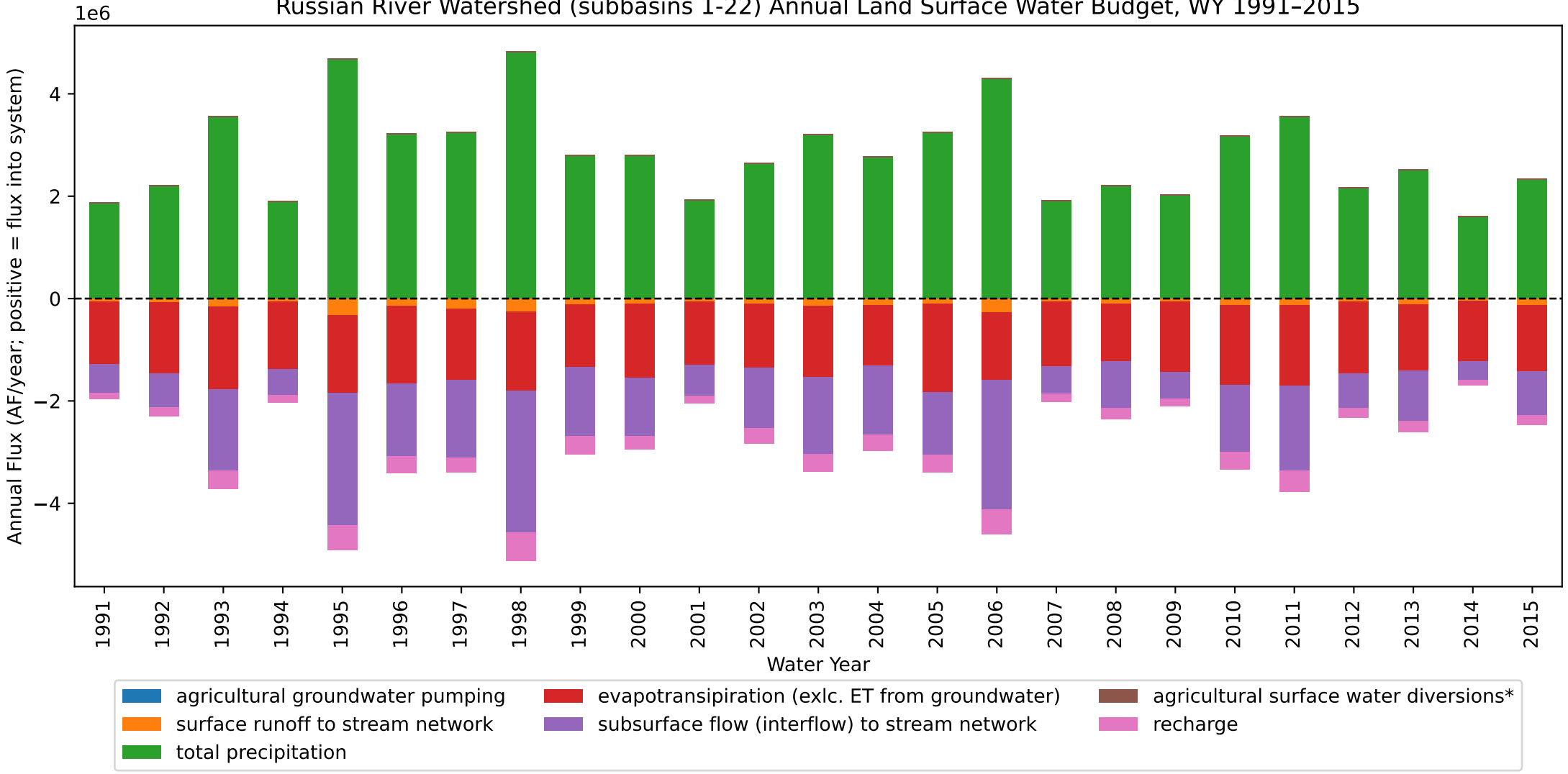
Russian River Watershed (subbasins 1-22) Annual Land Surface Water Budget, WY 1991-2015
