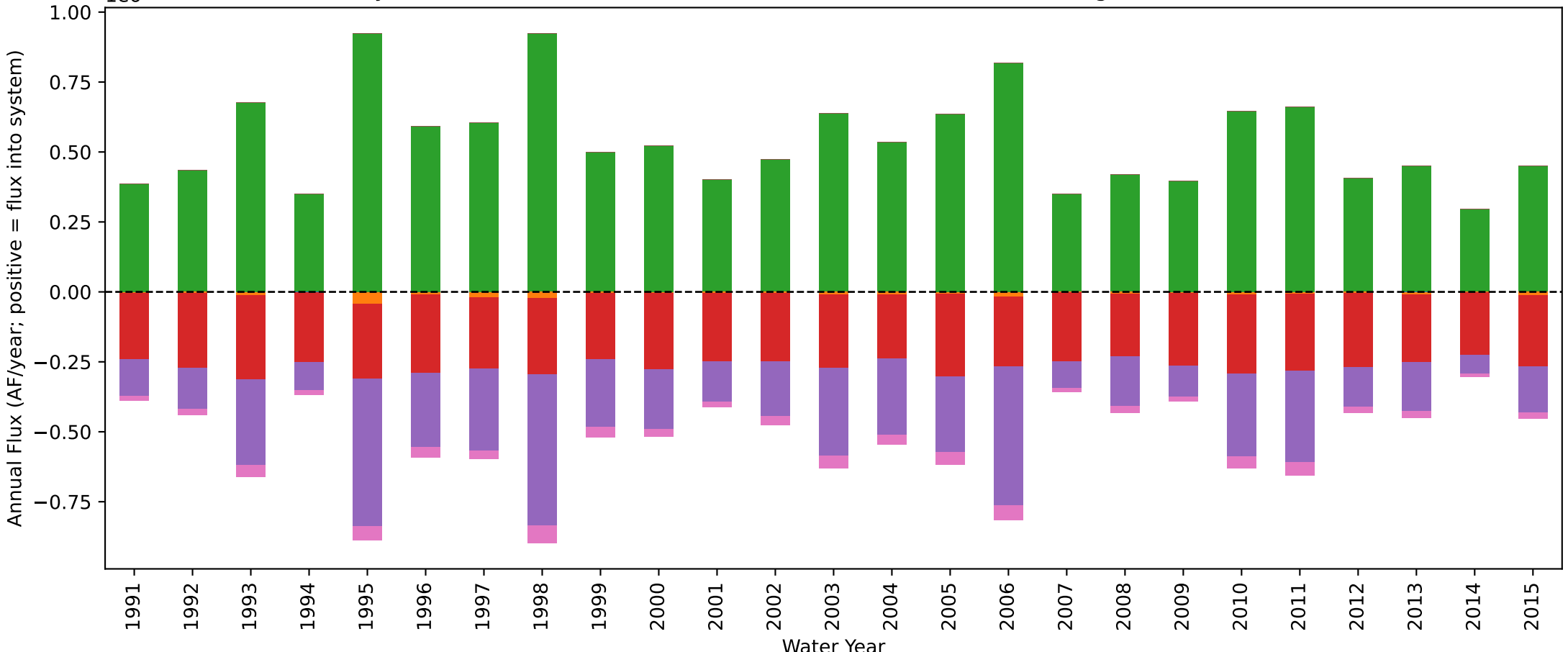
Dry Creek (subbasins 14-16, 22) Annual Land Surface Water Budget, WY 1991-2015
